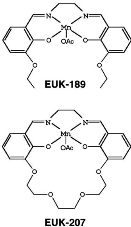
Fig. 1. Structures of EUK-189 and EUK-207.
